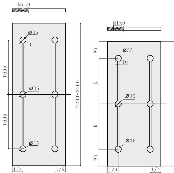
SLOTING DIMENSION
